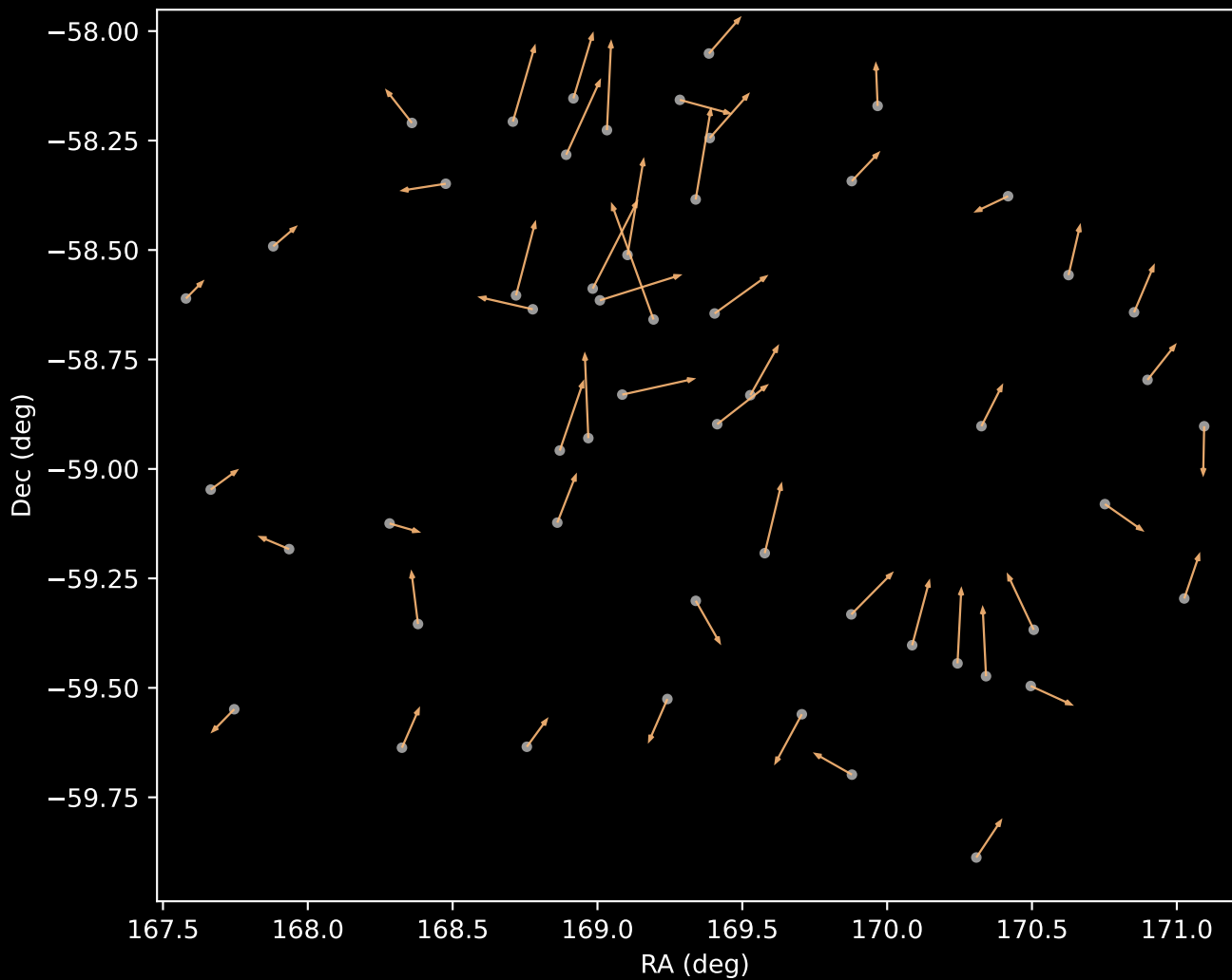
GALAH DR4 Cluster 3 Proper Motion Vectors (n=54)
