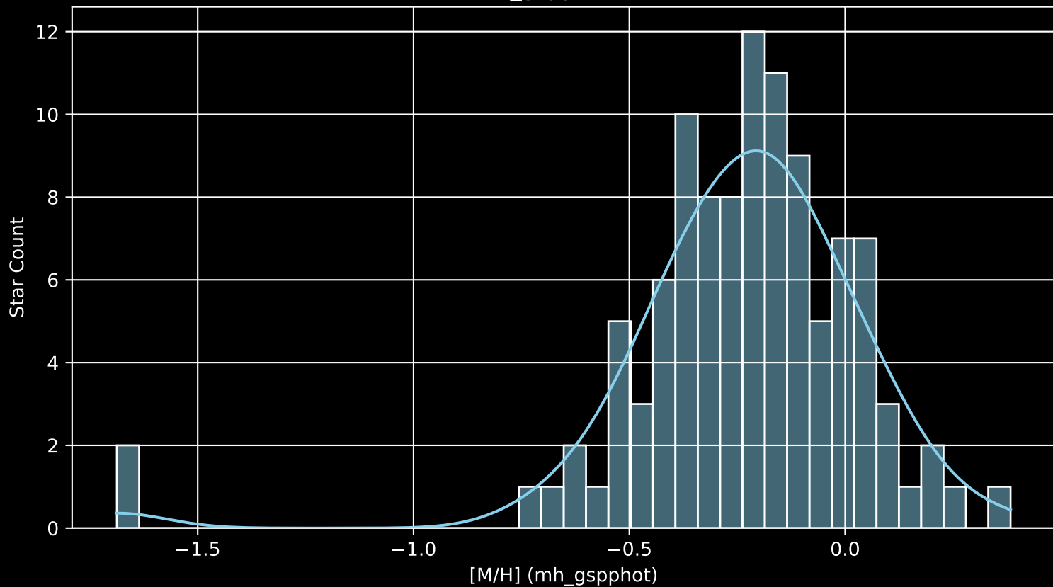
GALAH DR4 Field: [7213] [M/H] (mh_gspphot) (n= 106)
