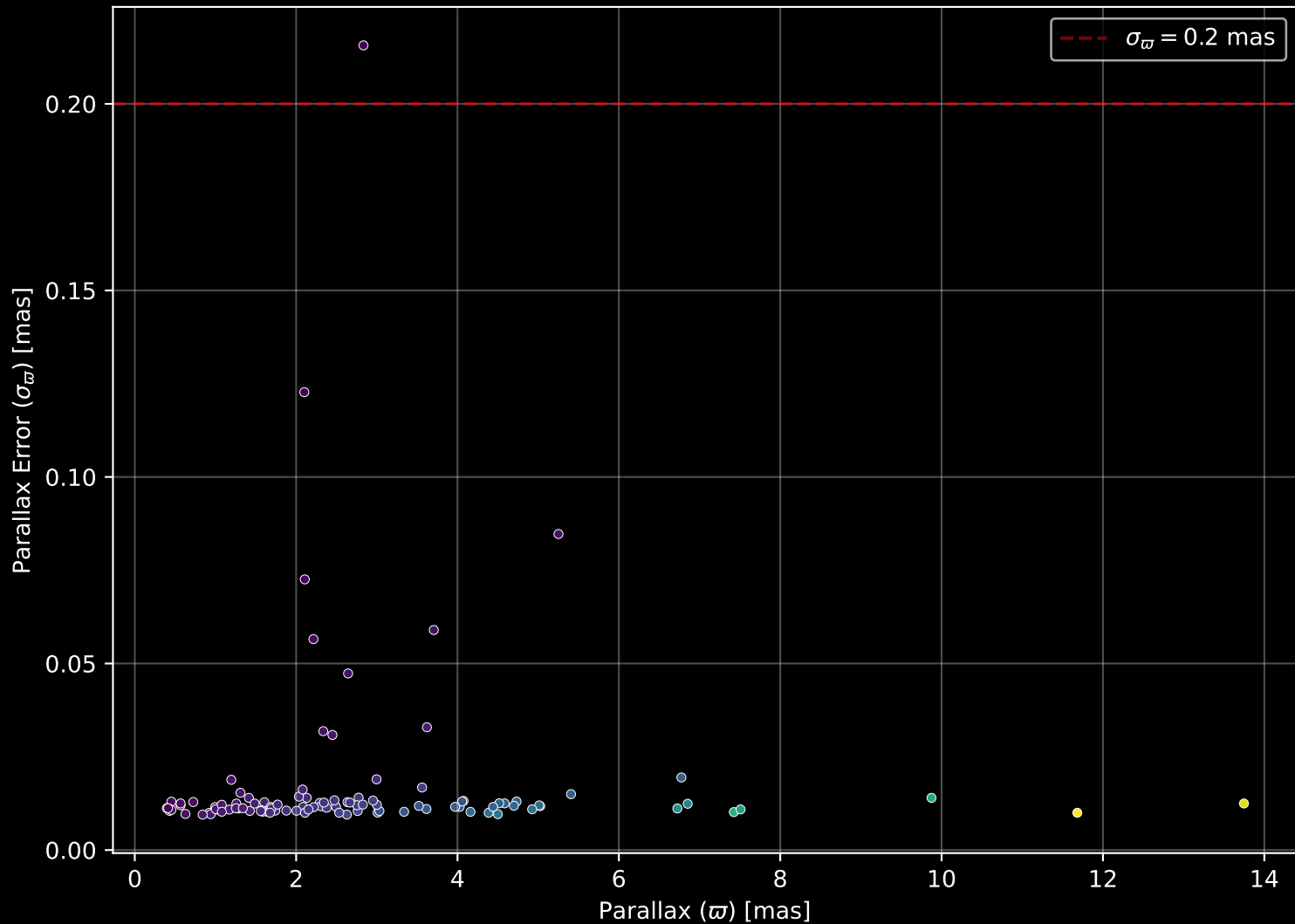
GALAH DR4 Field: [7213] Parallax Quality (n= 106)
