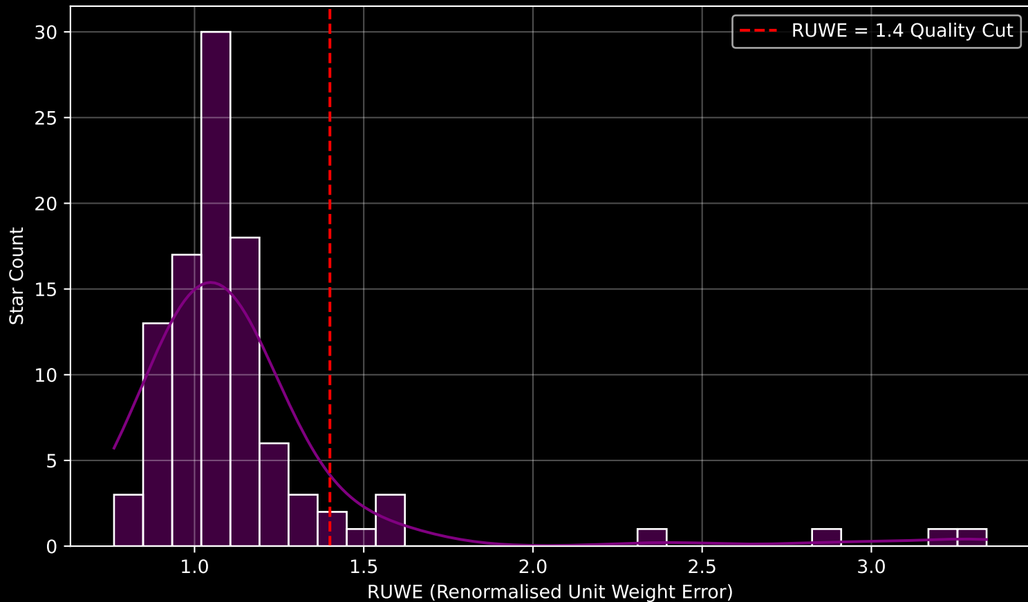
GALAH DR4 Field [7213] RUWE Distribution (n= 100)
