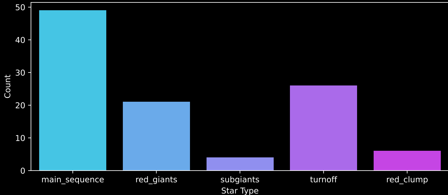
GALAH DR4 Field: [7213] Count plot of Star Type
