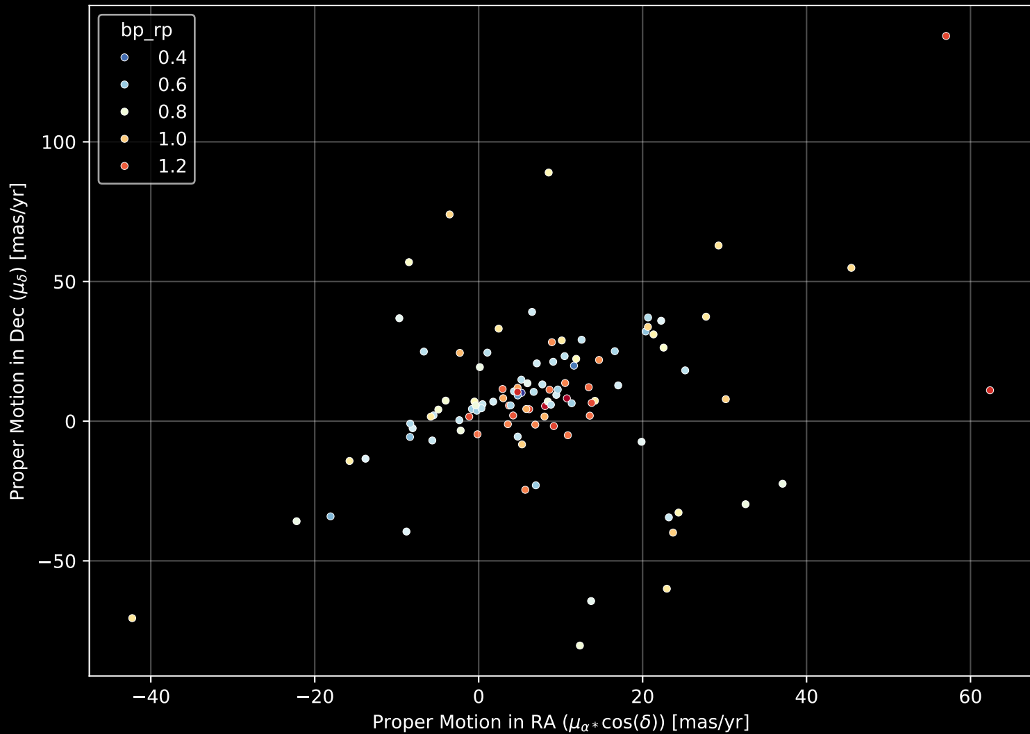
GALAH DR4 Field: [7213] Proper Motion Diagram (n= 106)
